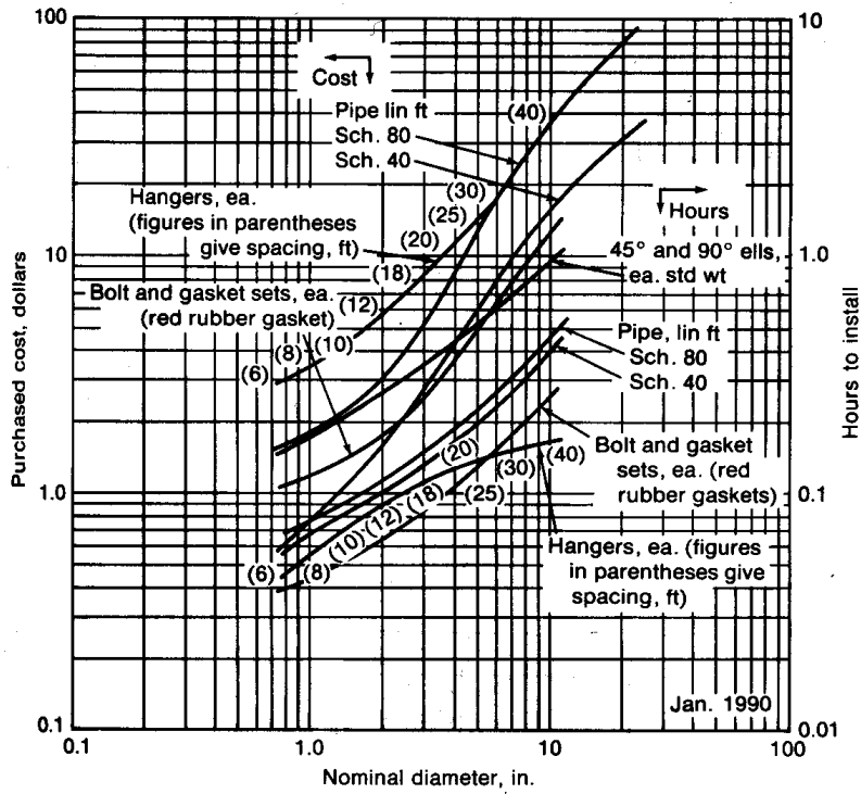
FIGURE 14-3 Cost and installation time for carbon-steel welded pipe and fittings.
