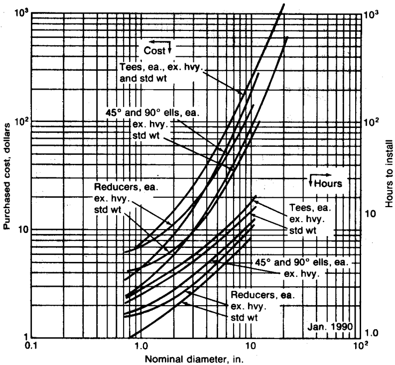
FIGURE 14-4 Cost and installation time for carbon-steel welded pipe fittings.
